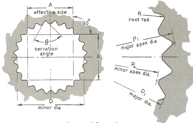
Internal Serrations
