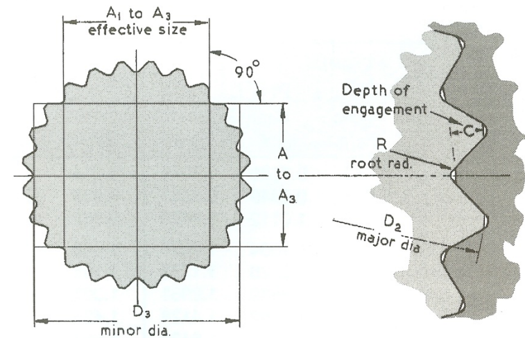
External Serrations
